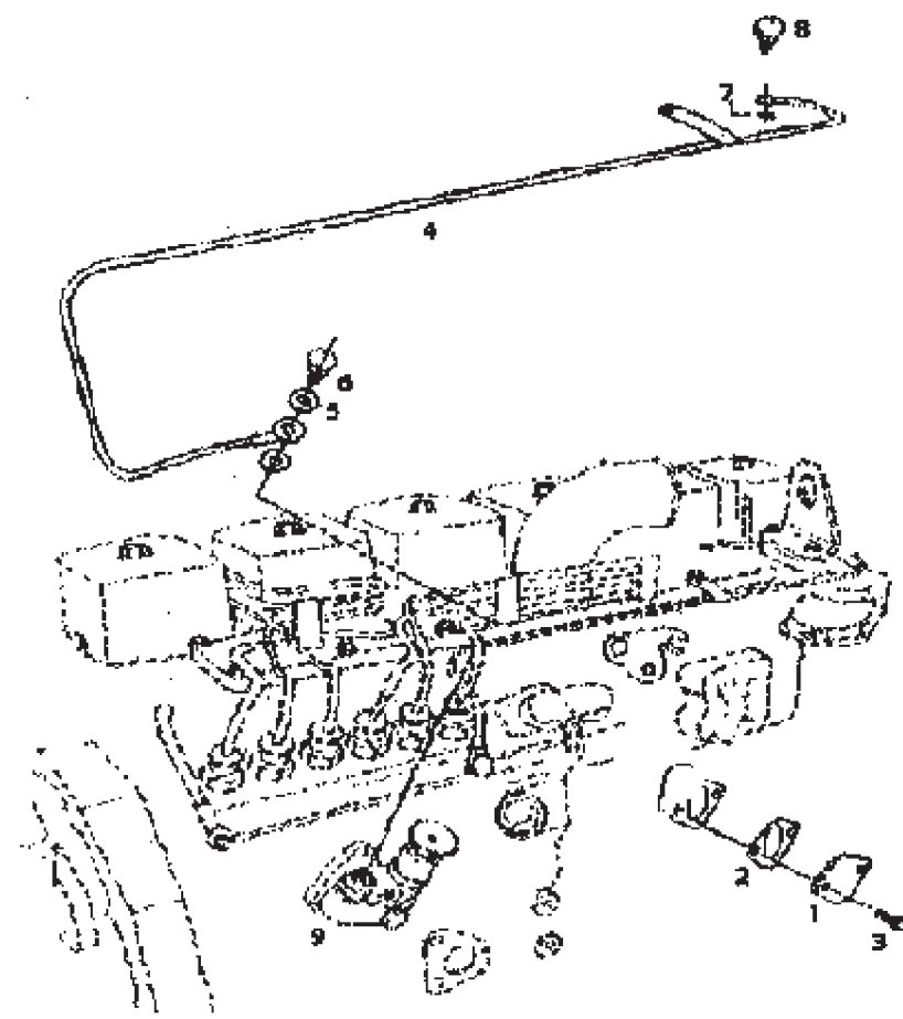
PUMP, FUEL LIFT
