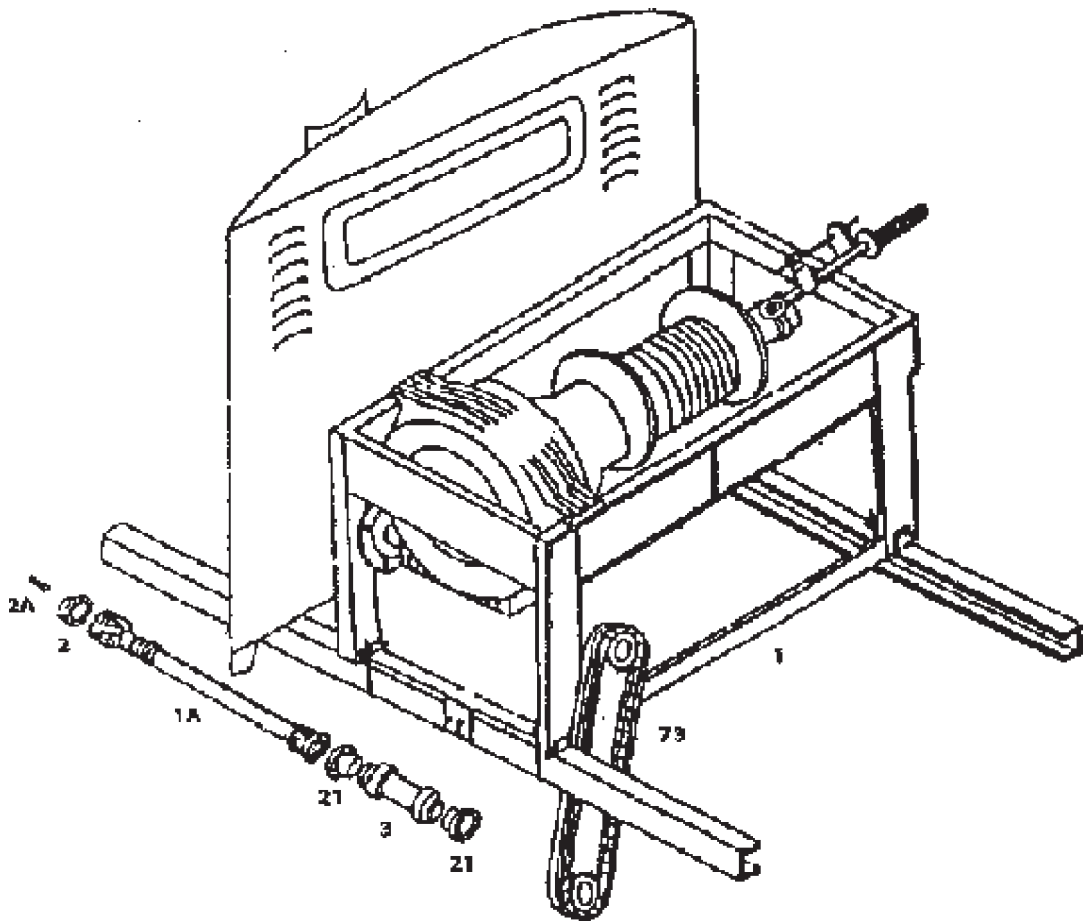
MECHANICAL WINCH
