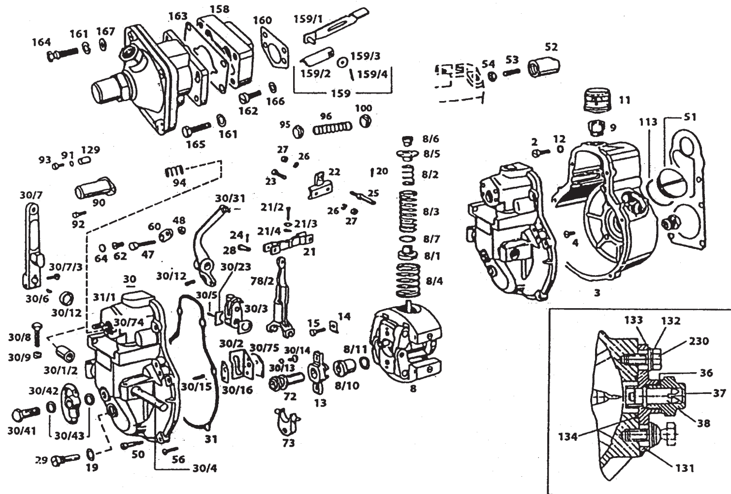
GOVERNOR (MICO)
