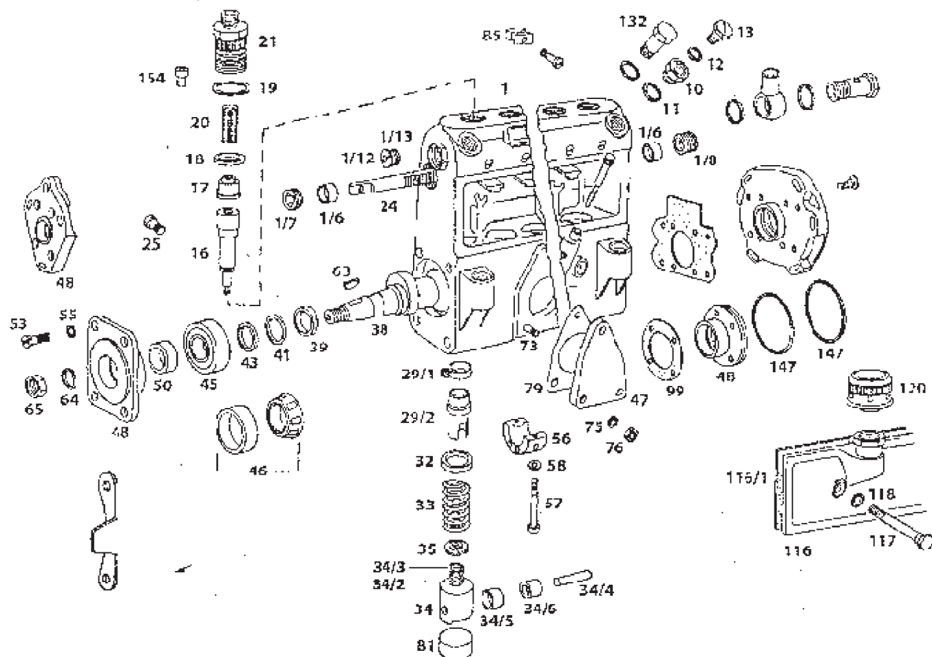
FUEL INJECTION PUMP (MICO)
