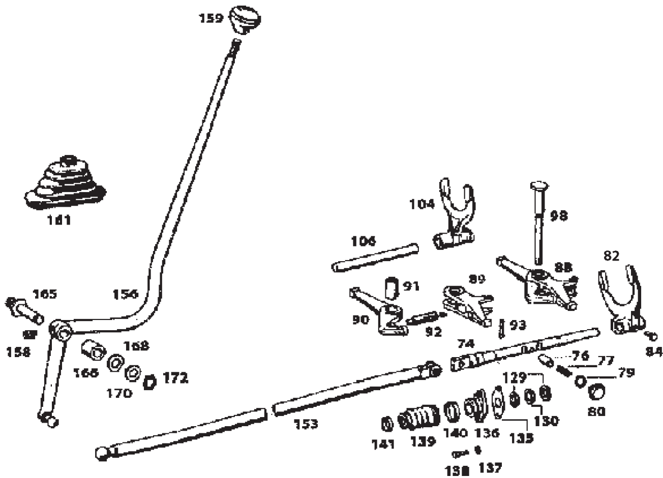
AUXILIARY GEAR BOX
