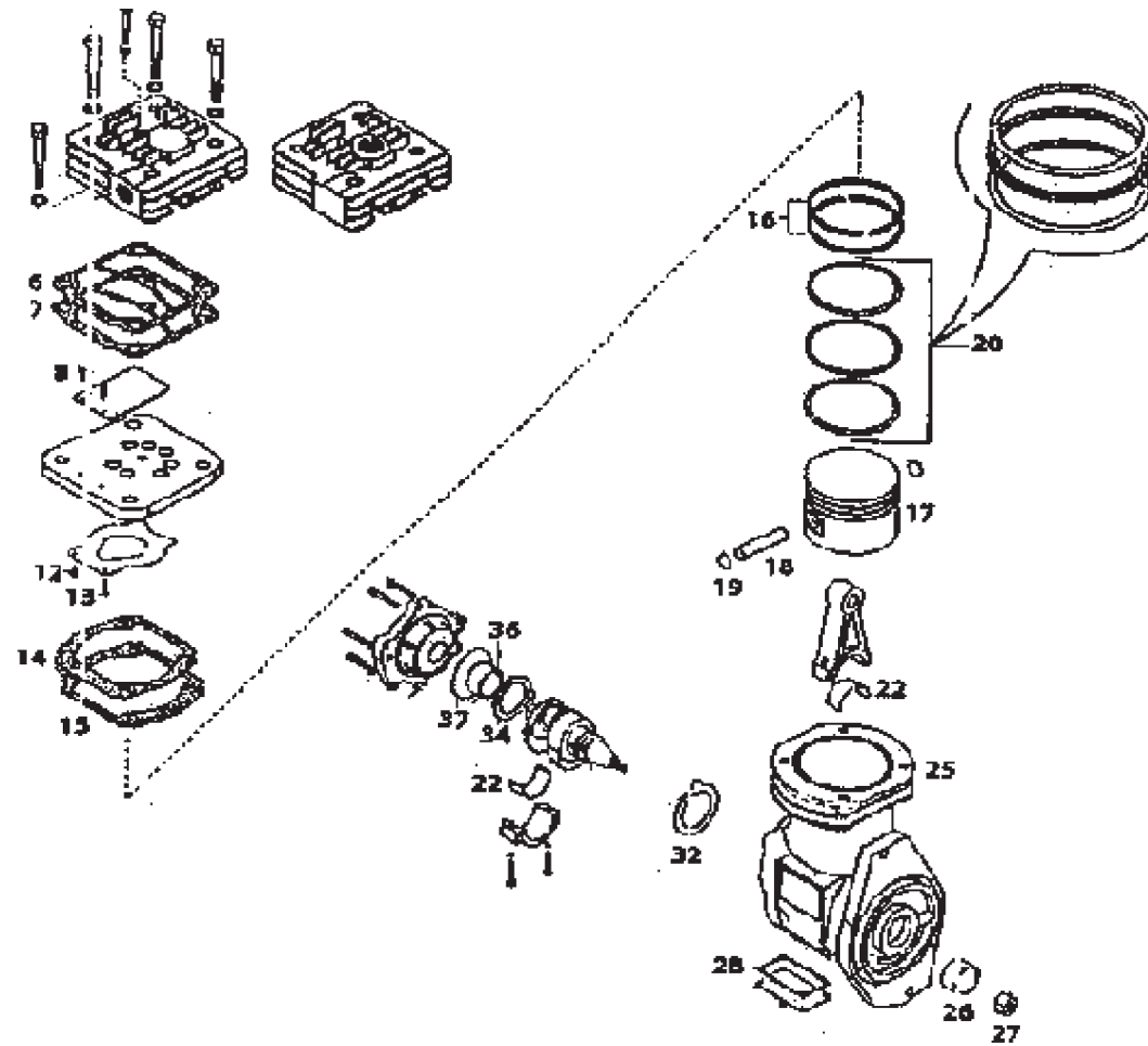
REPAIR KIT FOR AIR COMPRESSOR (SC 160)
