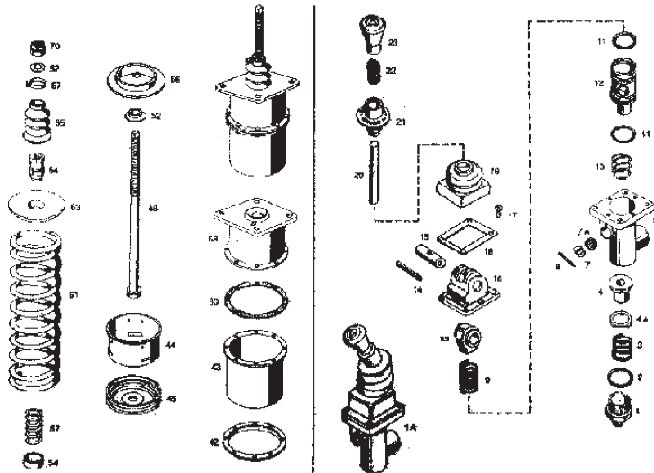
COMPONENTS OF SPRING BRAKE CHAMBER AND HAND BRAKE VALVE
