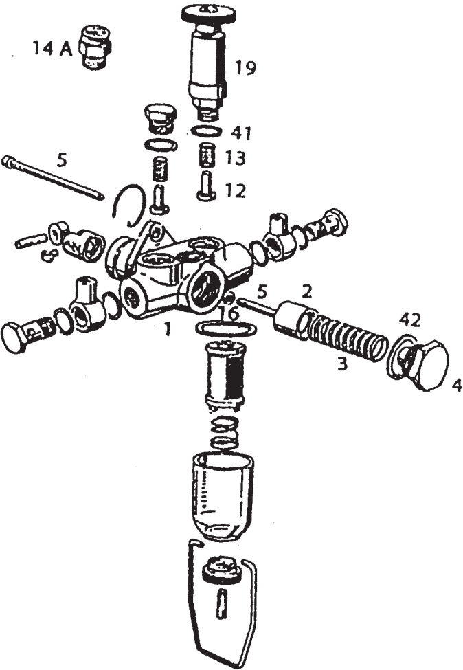
FEED PUMP (MICO)
