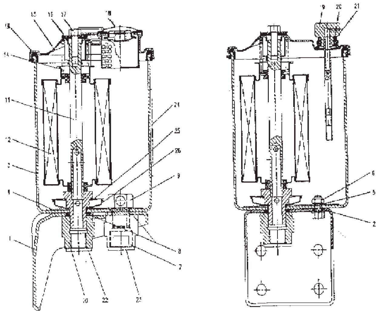
ASSY. HYDRAULIC TANK
