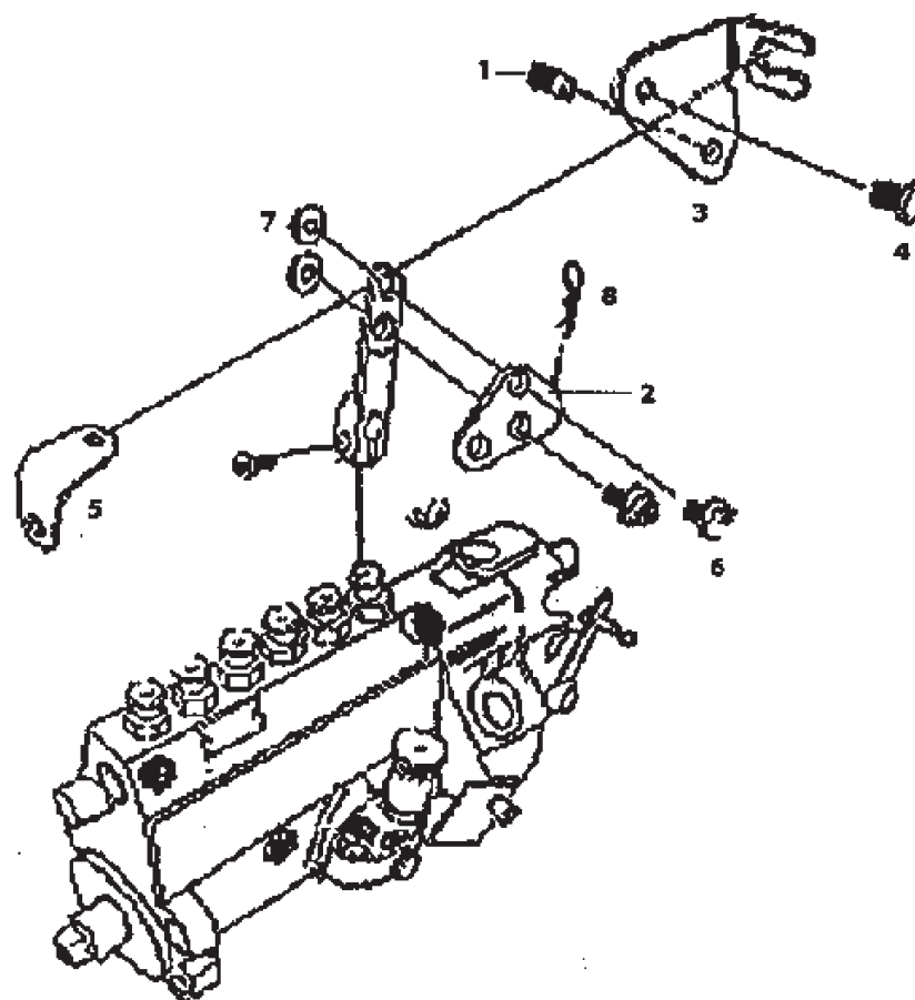
LEVER, FUEL SHUT OFF
