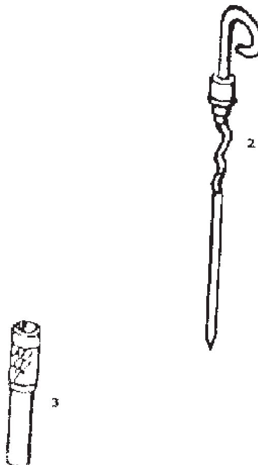
OIL LEVEL GAUGE
