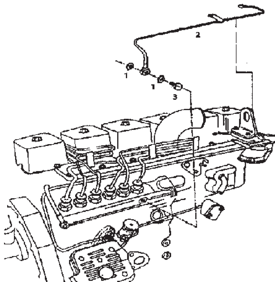
PLUMBING FUEL FILTER
