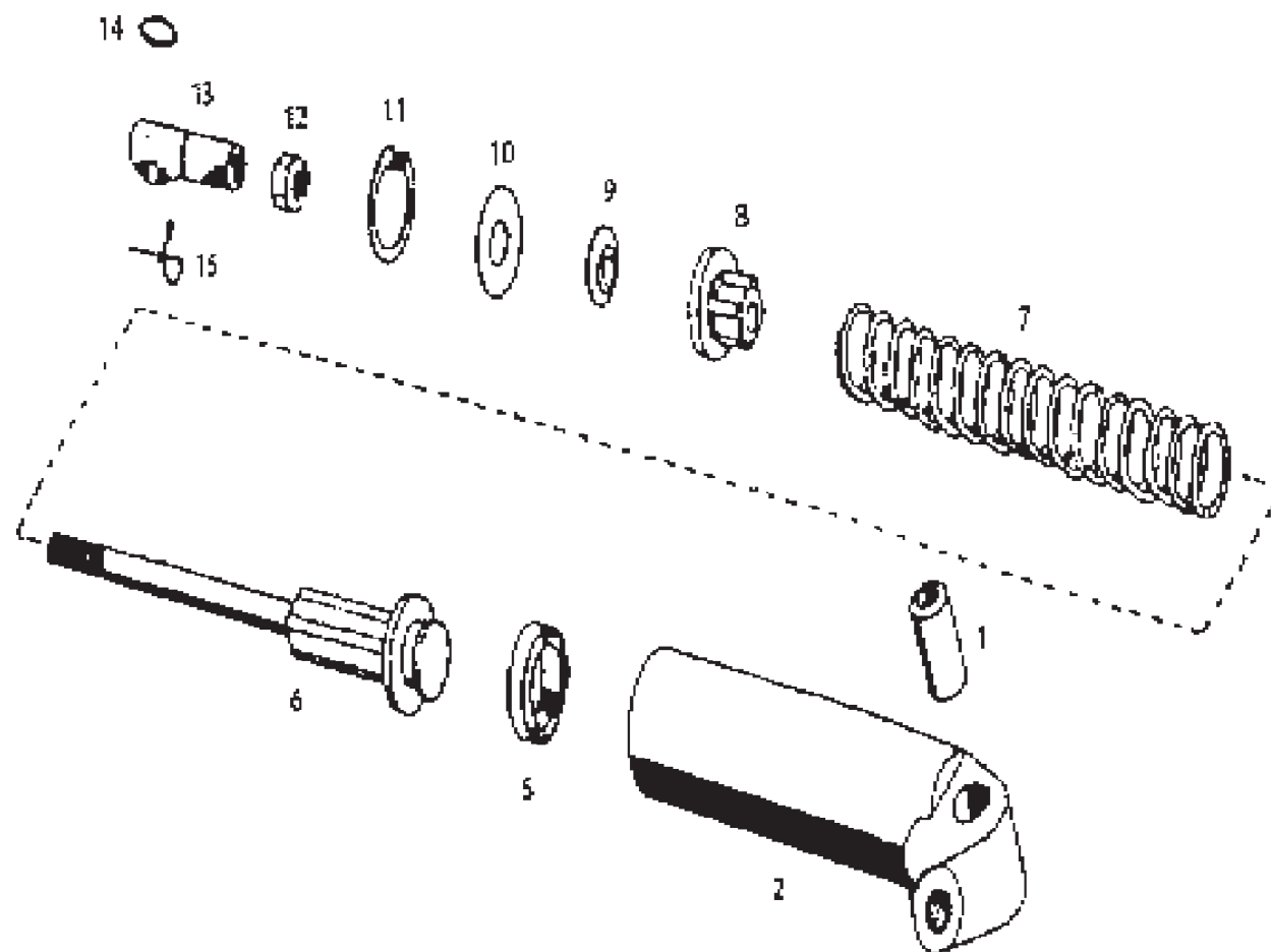
AGGREGATE OF ENGINE BRAKE
