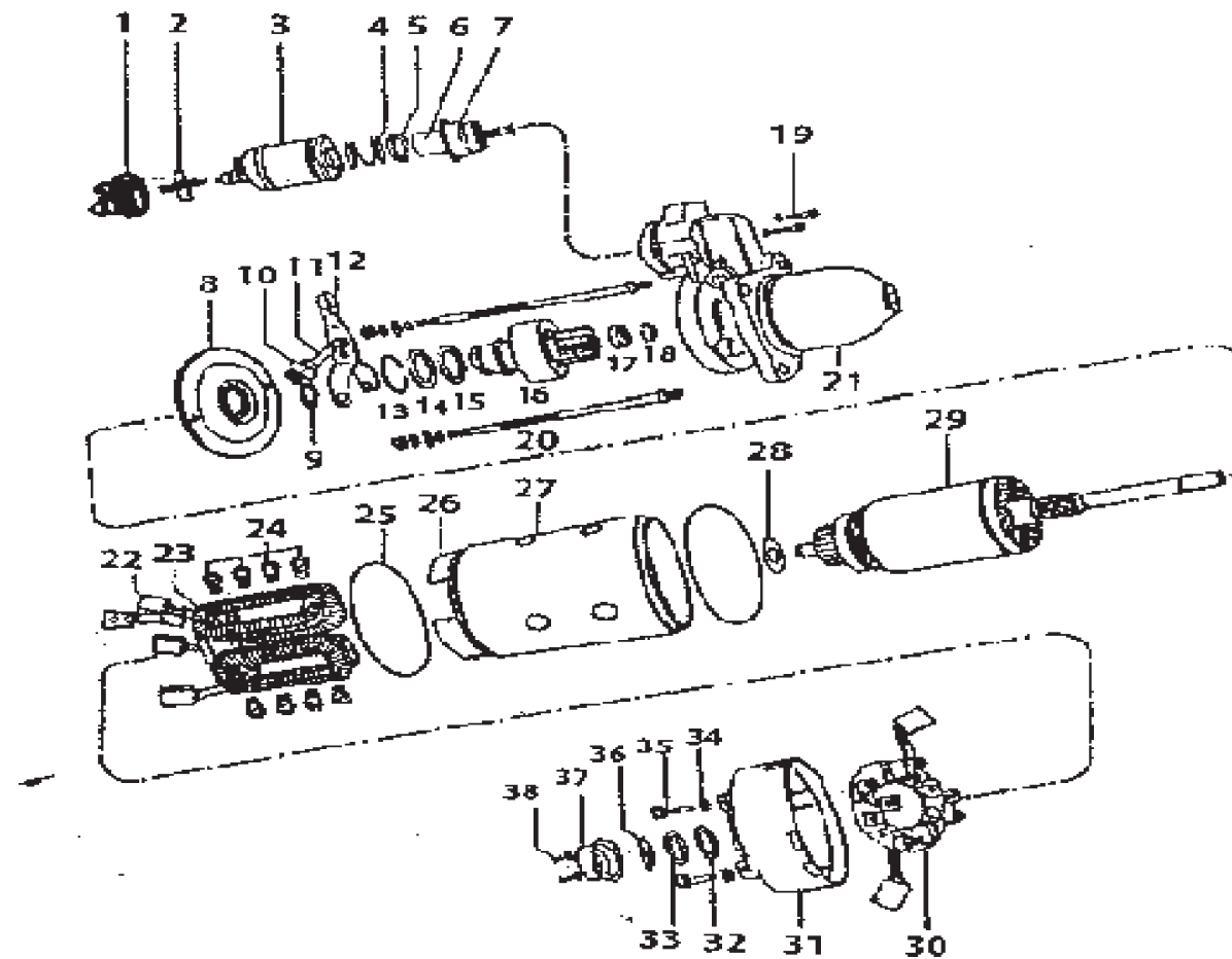
COMPONENT DETAILS OF STARTER MOTOR
