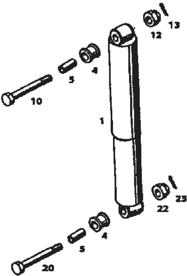
REAR SHOCK ABSROBERS AND MOUNTINGS
