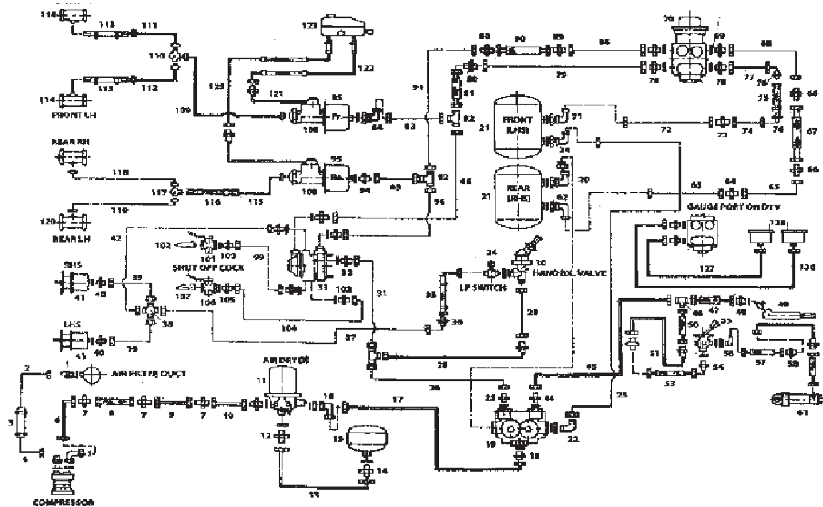
BRAKE LINES
